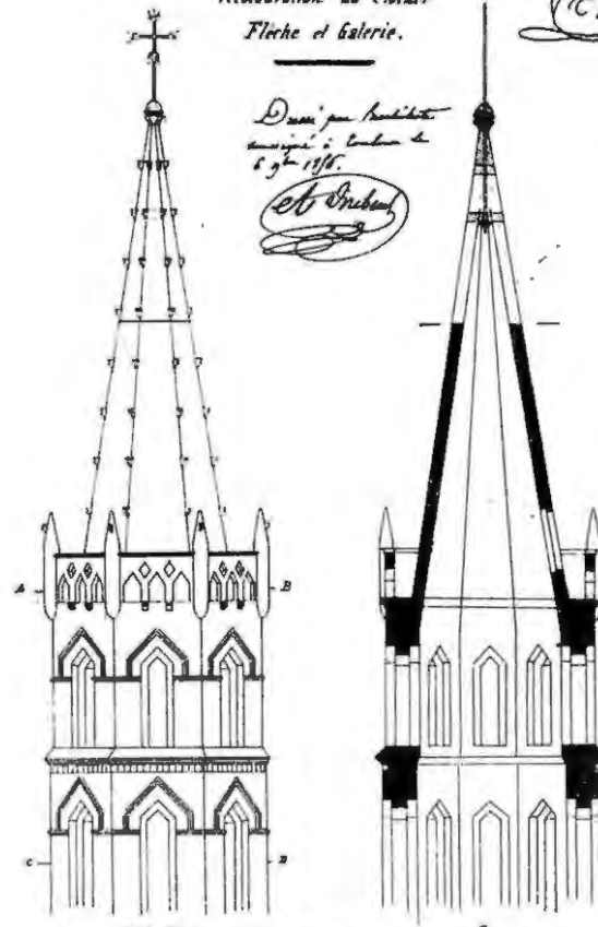
Elevation.
